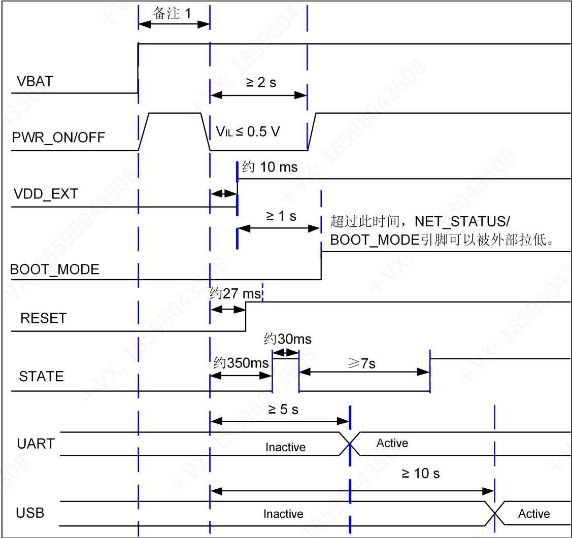
Figure 16. 开机时序图
